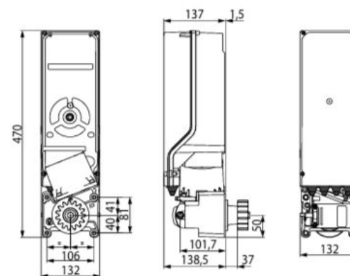
MOTOR WITH INTEGRATED CONTROL UNIT TW90/600/HS - TW90/800 - TW90/800/R
